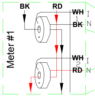
Diagram 1. Current Transformers installed inside tenant breaker panel. Note: Conductor for each LINE 2 must be run reverse (backwards) through CT.
